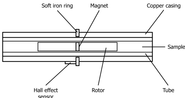
FIG. 1 Viscosity Cell
