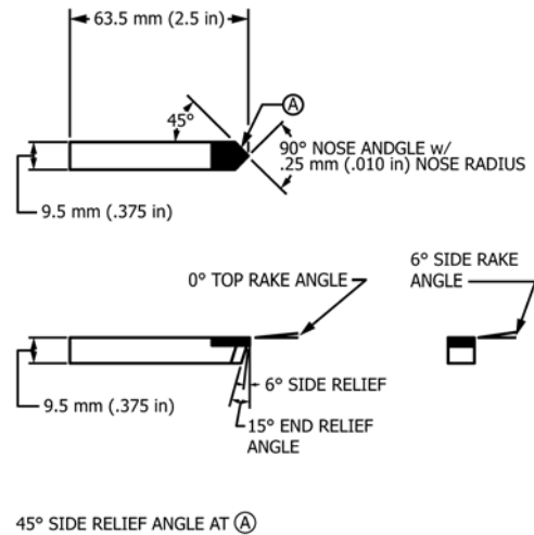
FIG. 4 Tool Bit
