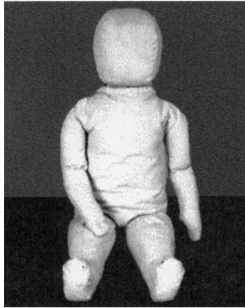
FIG. 12 CAMI Newborn Dummy 7.5 lb (3.4 kg)
