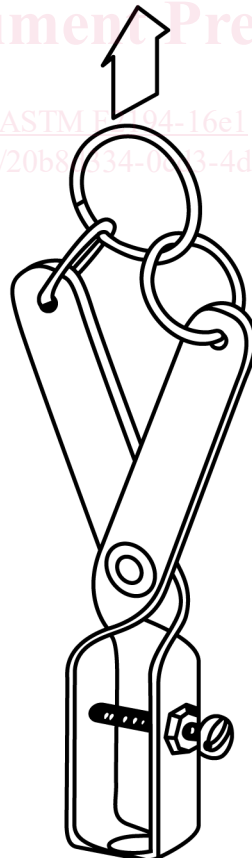
FIG. 78 Sketch of Clamping Device
