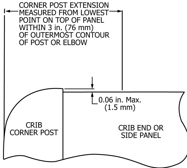
FIG. 34 Corner Post Extension
