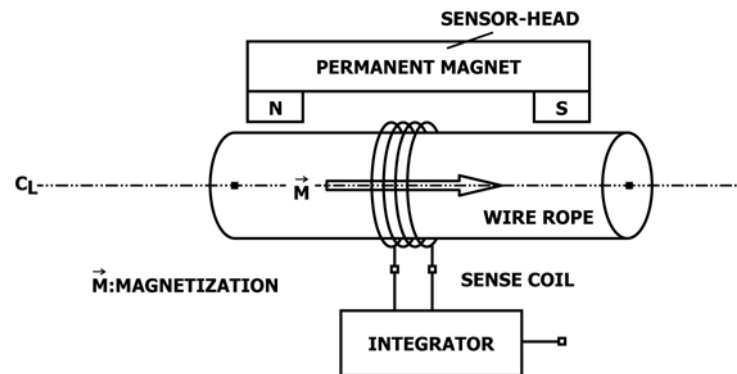
FIG. 1 Schematic Representation of a Permanent Magnet Equipped Sensor-Head Using a Sense Coil to Measure the Loss of Metallic Cross-Sectional Area
