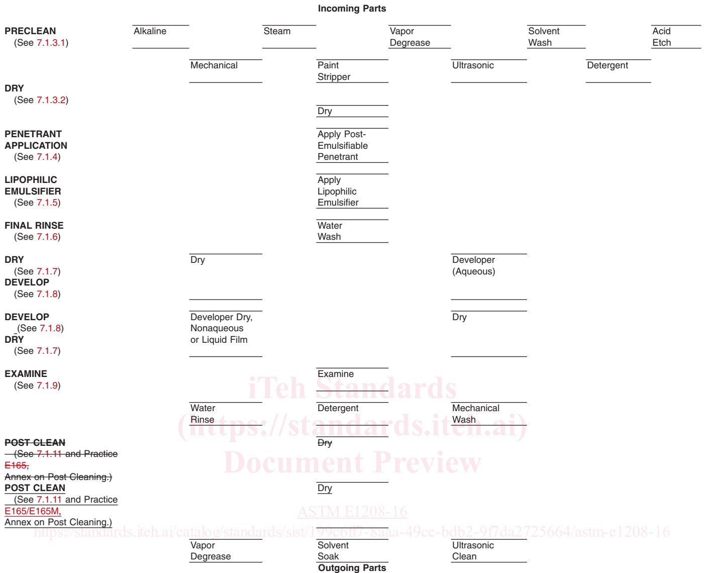
FIG. 1 General Procedure Flowsheet for Fluorescent Penetrant Examination Using the Lipophilic Post-Emulsification Process
