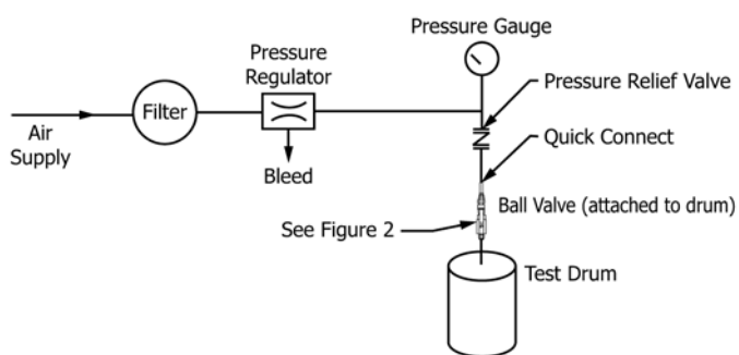
FIG. 1 Apparatus for Procedure A
