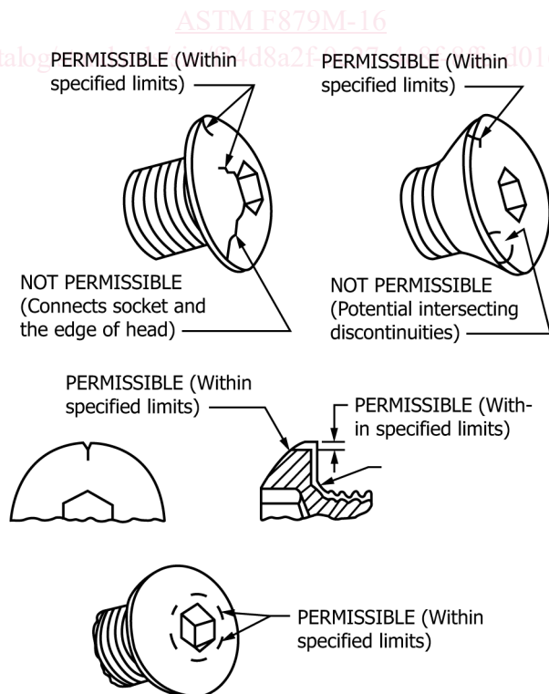
FIG. 1 Head Discontinuities (See 10.2.1.1 and 10.2.1.2 )
