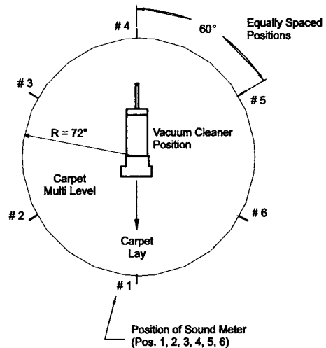
FIG. 2 Sound Test Pattern for Uprights
