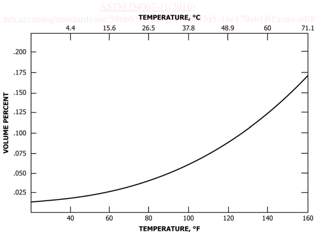
FIG. A1.1 Solubility of Water in Toluene
