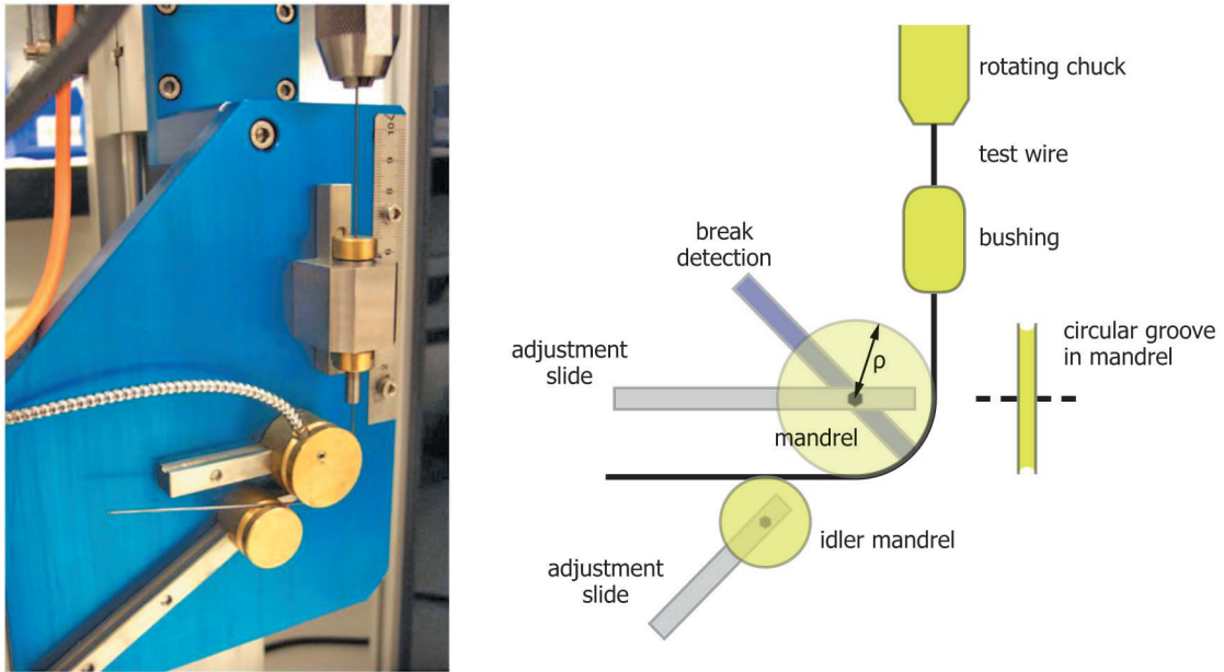
FIG. 3 Guided Rotating Bending Fatigue Apparatus
