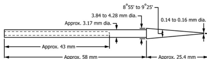
FIG. 2 Standard Needle
