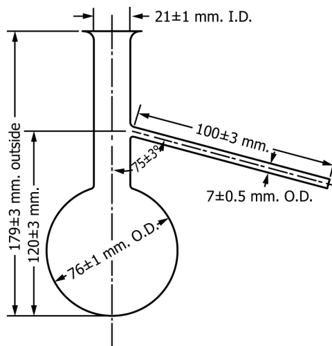
FIG. 1 Distillation Flask
