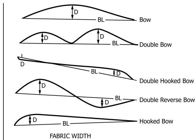
FIG. 1 Typical Bow Conditions
