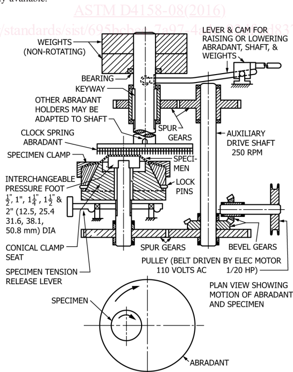
FIG. 1 Schematic Diagram of Uniform Abrasion Testing Machine
