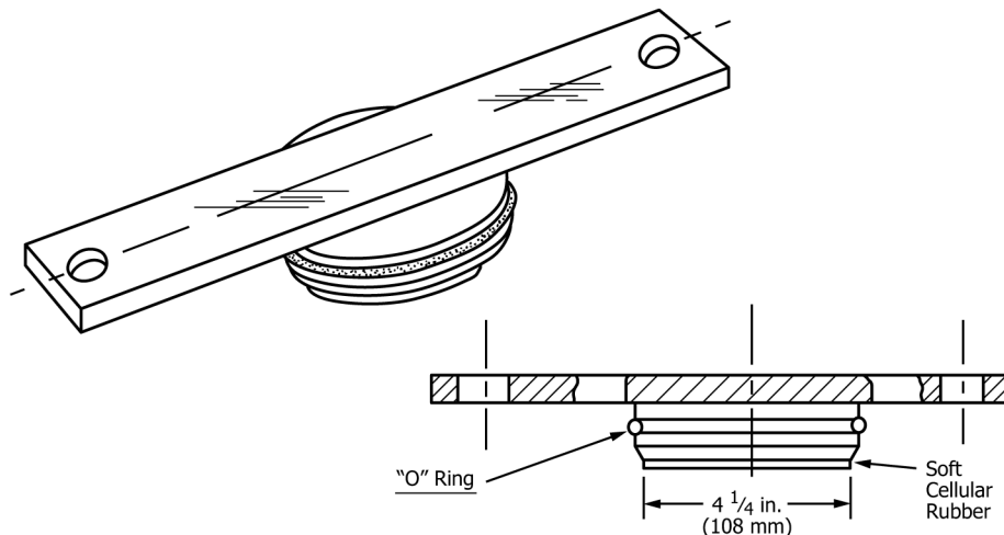
FIG. 2 Specimen Holder
