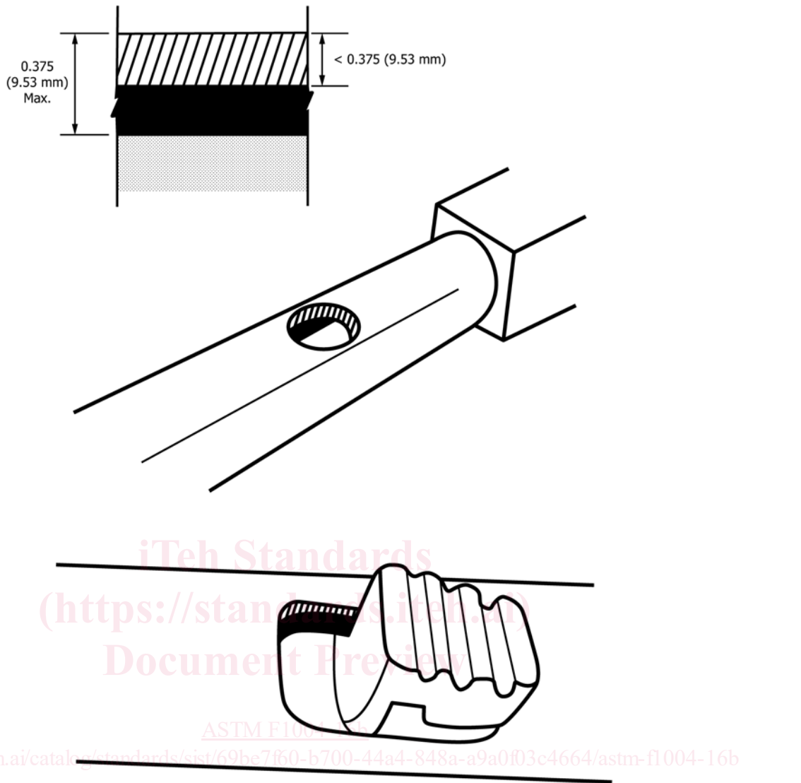
FIG. 1 Openings
