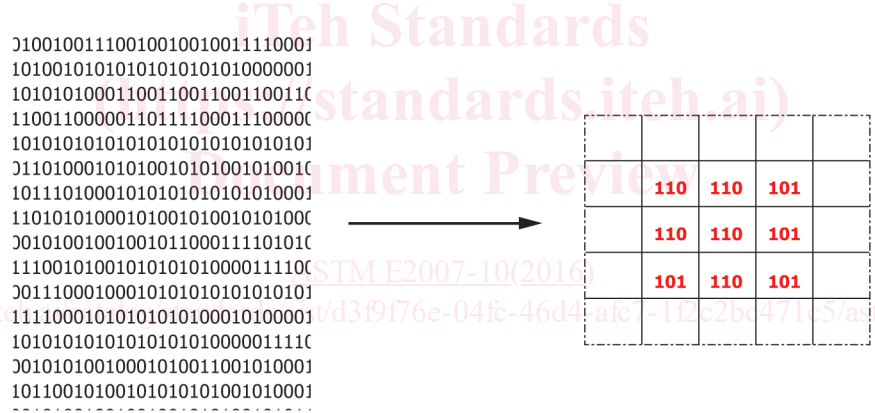
FIG. 4 Assignment of Binary Data to a Pixel Matrix (3-bit depth illustrated)
