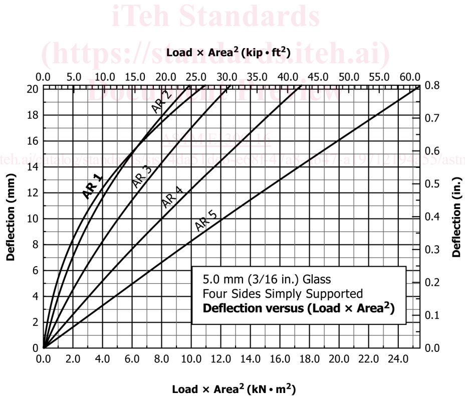
FIG. A1.6 (upper chart) Non-Factored Load Chart for 5.0 mm ( \frac{3}{16} in.) Glass with Four Sides Simply Supported (lower chart) Deflection Chart for 5.0 mm ( \frac{3}{16} in.) Glass with Four Sides Simply Supported
