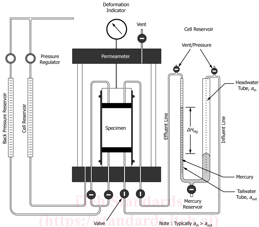
FIG. 4 Constant Volume – Falling Head System, Method F (56)
