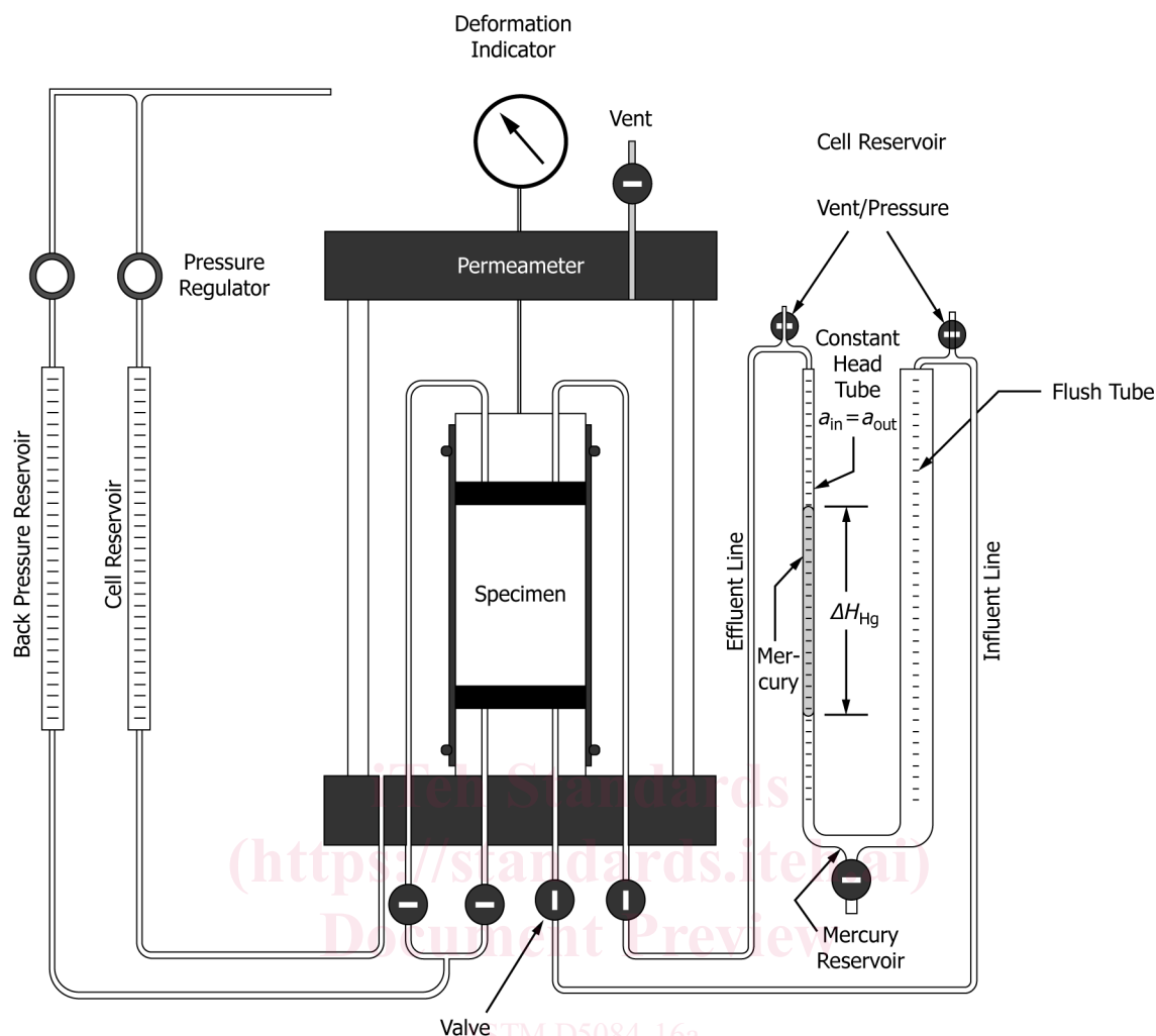
FIG. 2 Constant Volume – Constant or Falling Head System, Method E or F (56)
