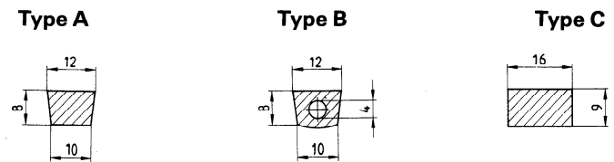
Figure 1 — Cross-sections of gaskets
