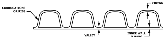
FIG. 1 Typical Triple-Corrugated Double Wall Pipe Profile
