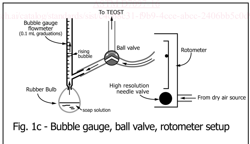
FIG. 1 Bubble Gauge
