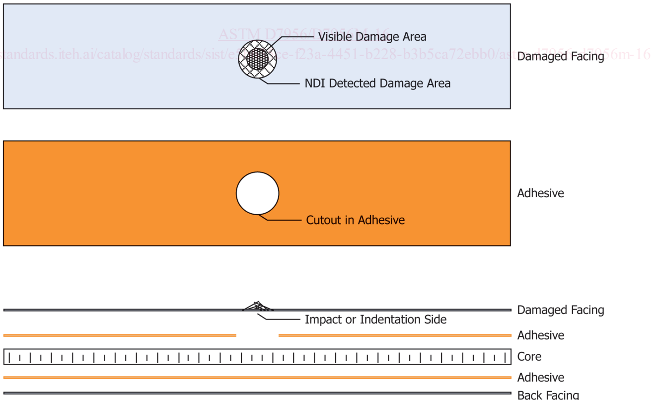
FIG. 1 Sandwich Specimen Assembly
