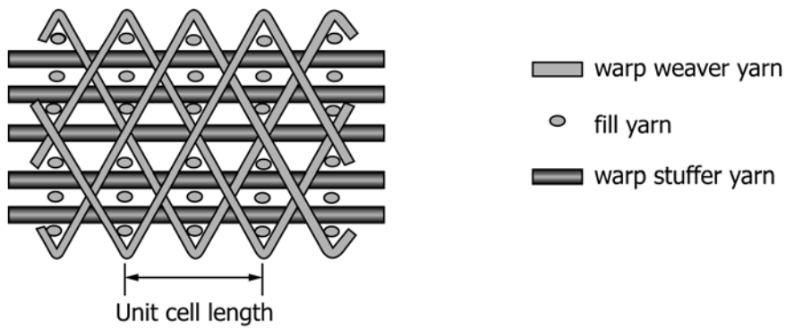
FIG. 3 Smallest Unit Cell Length for Through-Thickness Angle-Interlock Weave
