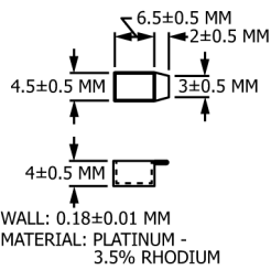
FIG. 1 Combustion Boat, Size A
