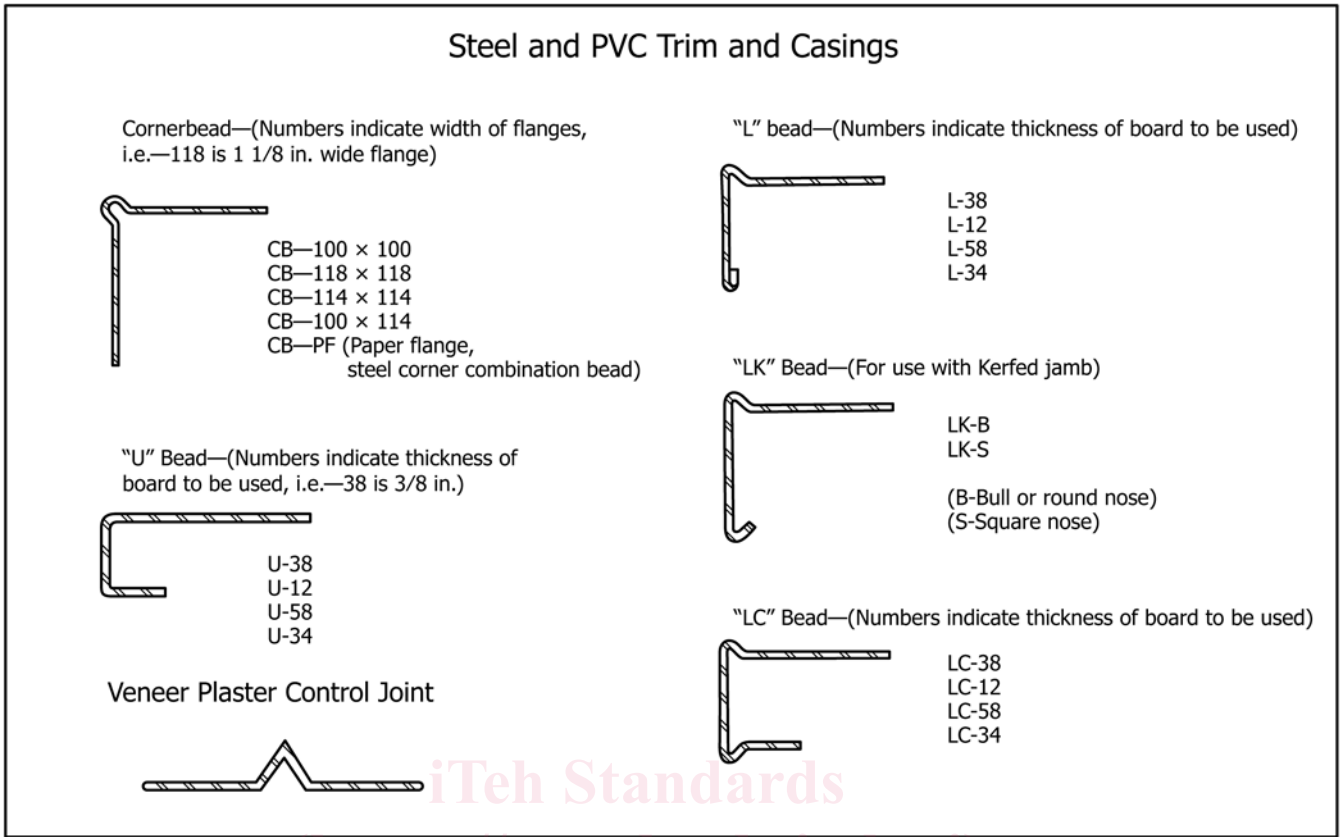
FIG. 1 Accessories
