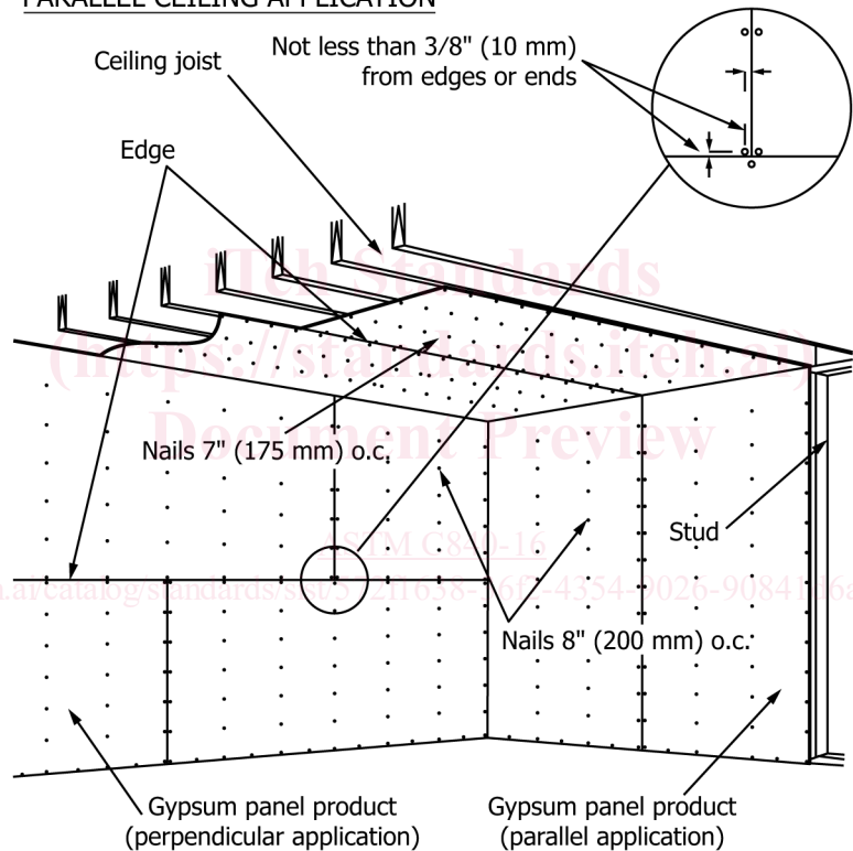
FIG. 2 Single Nailing
