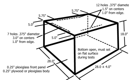
FIG. 3 Draft Enclosure
