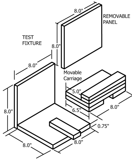
FIG. 1 Mini-Mock-Up Tester
