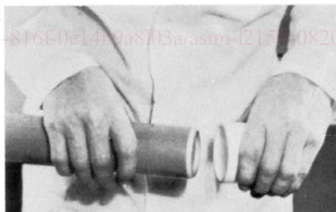
FIG. X3.2 Tube Entering Dry Fitting
