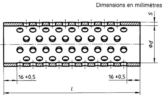
Figure 1 — Tube cylindrique
