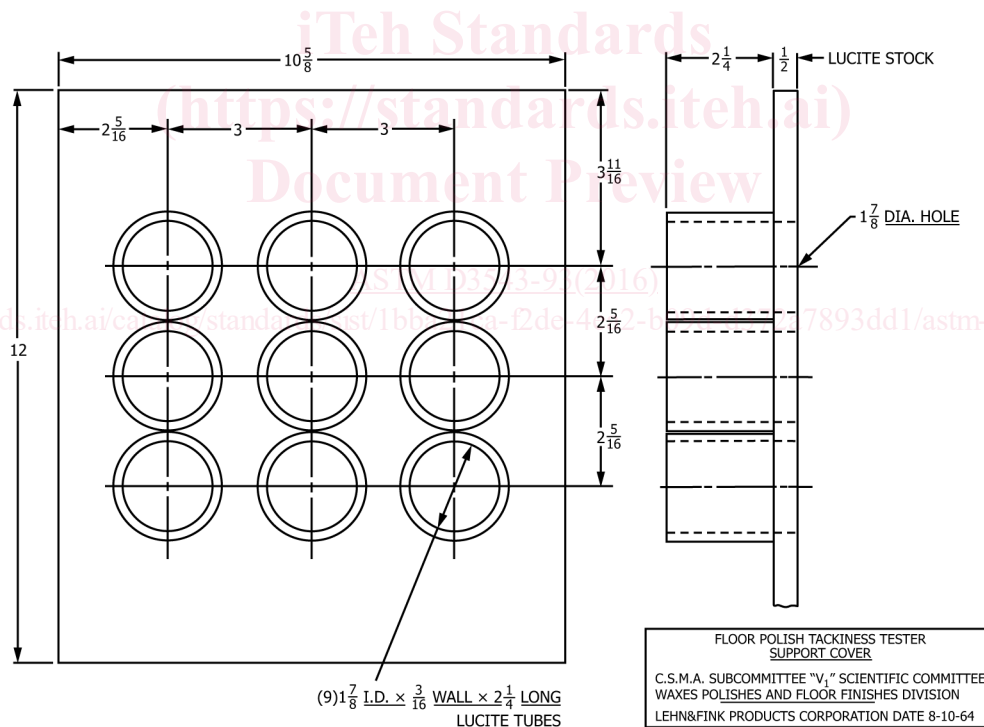
FIG. 2 Support Cover
