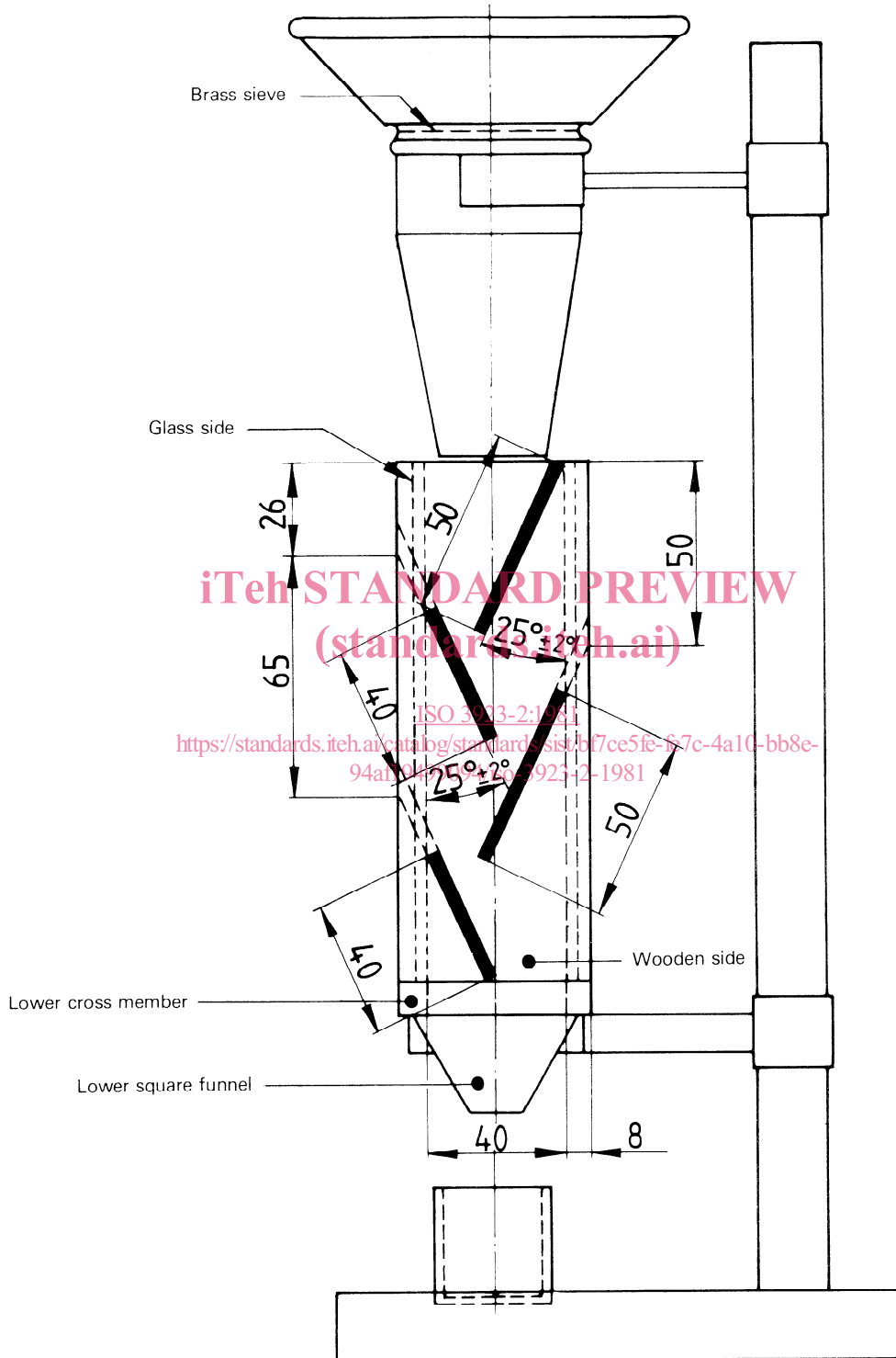
Figure 2 — Test apparatus — Side view
