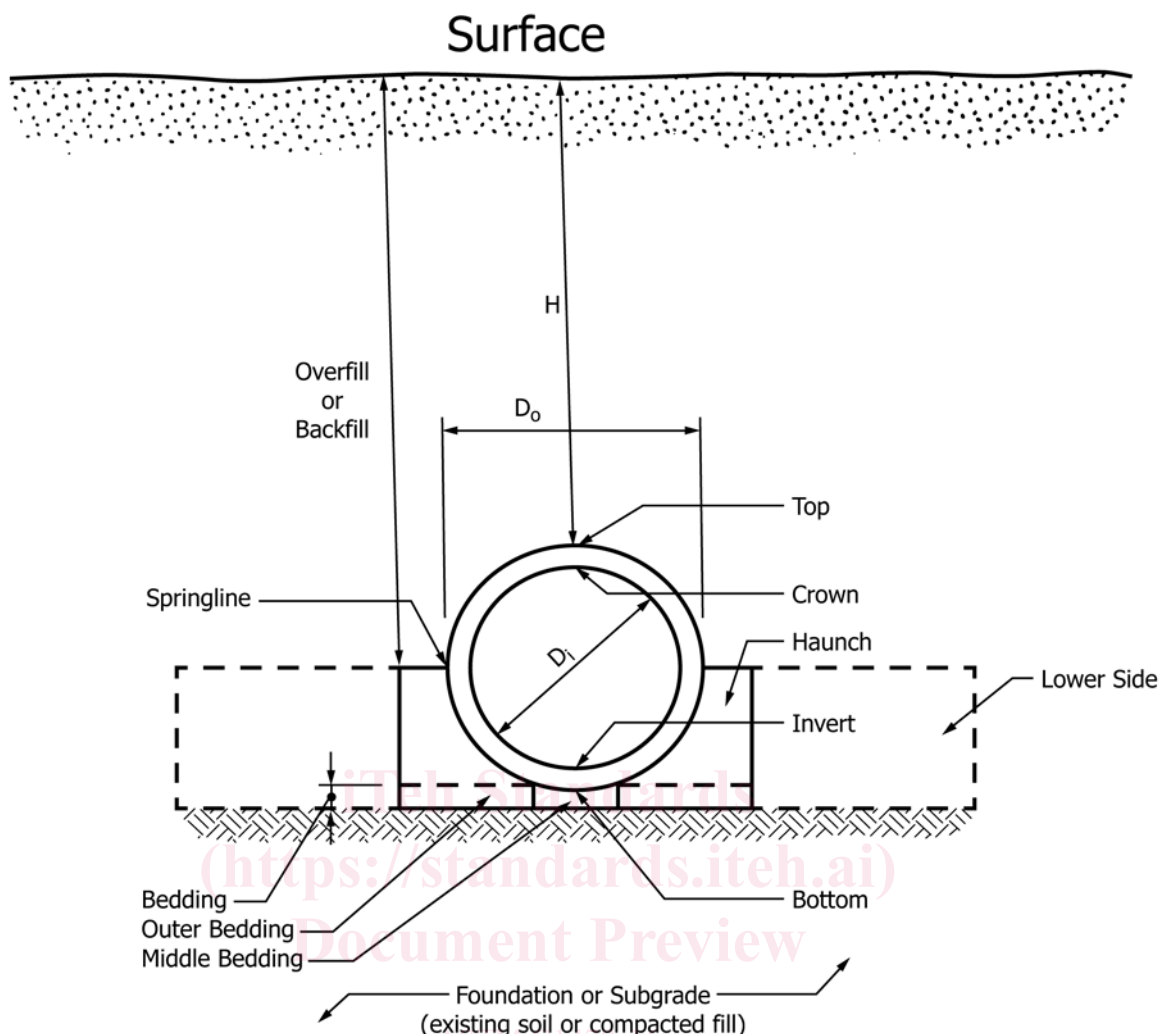
FIG. 1 Pipe/Installation Terminology
