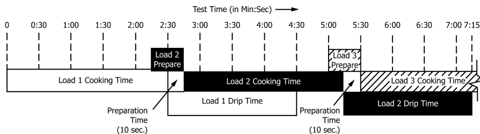
FIG. 2 Sequence of Stir-Up Cook Test (Not to Scale)
