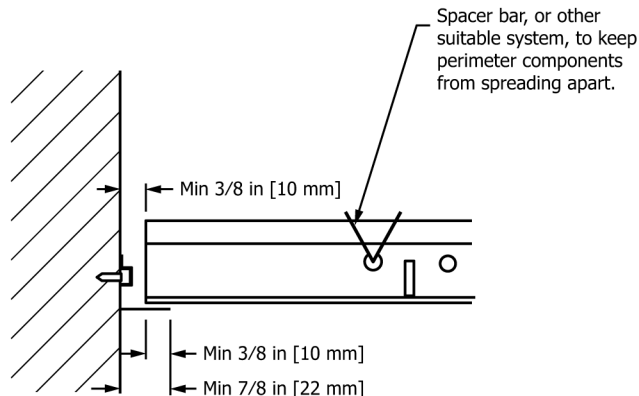
FIG. 12 Category C Treatment of Cross Runners, Main Runners, and Wall Closures at Terminal Ends
