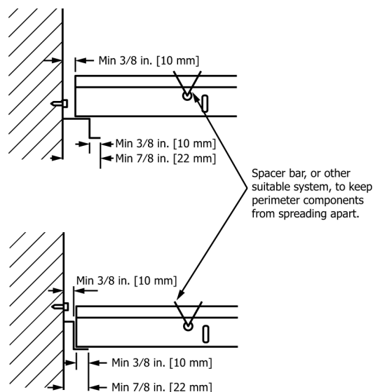
FIG. 23 Category C Treatment of Cross Runners and Main Runners at Terminal Ends When Using Reveal (Shadow) Edge Wall Closures
