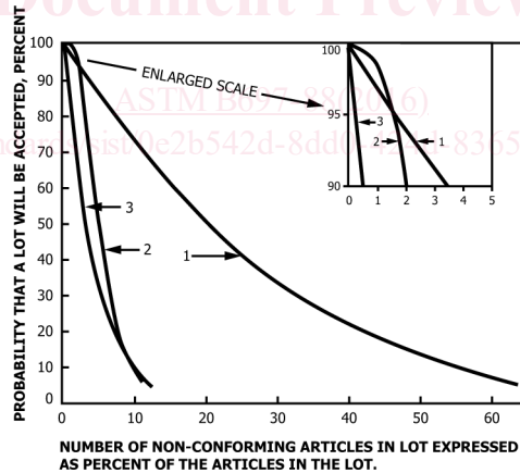
FIG. 4 Operating Characteristic Curves of Three Single Sample Attributes Sampling Plans
