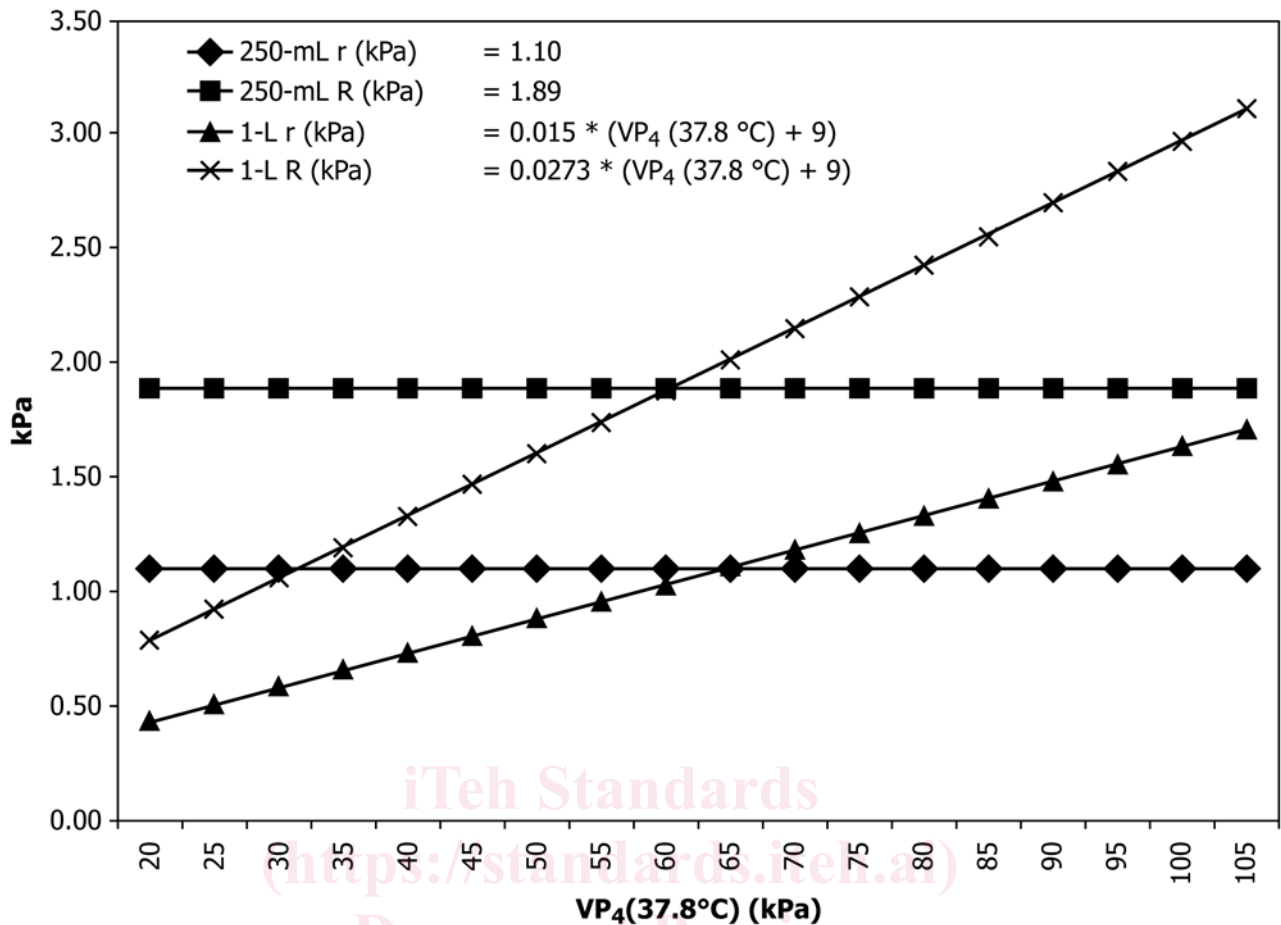
FIG. 1 Plot of VP 4 (37.8 °C) Precision (kPa) by Container Size at Nominal VP 4 (37.8 °C) (kPa) Values Determined
