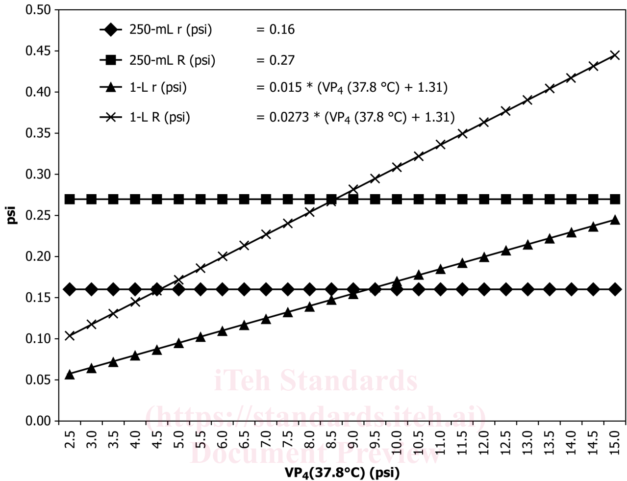
FIG. 2 Plot of VP 4 (37.8°C) (37.8 °C) Precision (psi) by Container Size at Nominal VP 4 (37.8°C) (37.8 °C) (psi) Values Determined
