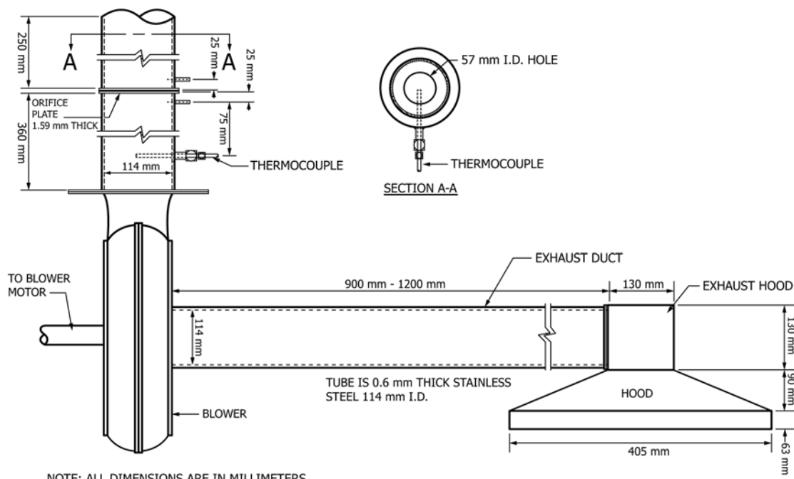
FIG. 3 Exhaust System
