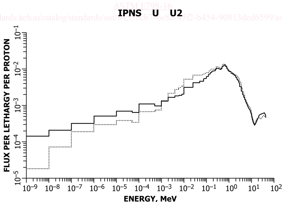
NOTE 1—Neutron flux spectrum at the Intense Pulsed Neutron Source of ANL with 500 MeV protons and a depleted uranium target. The solid line is calculated and the dashed is an adjusted spectrum based on radiometric dosimetry. (Data from Ref (12); (12).)
