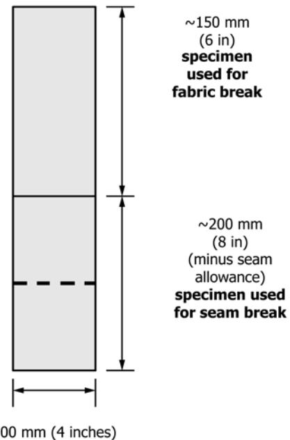
FIG. 1 Seamed Specimen Removed from Manufactured Item
