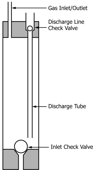
FIG. 3 Air/Gas Displacement Pump
