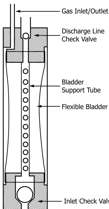
FIG. 5 Bladder Pump—Squeeze Type
