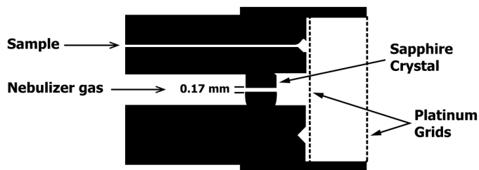
FIG. 5 Grid Nebulizer 6
