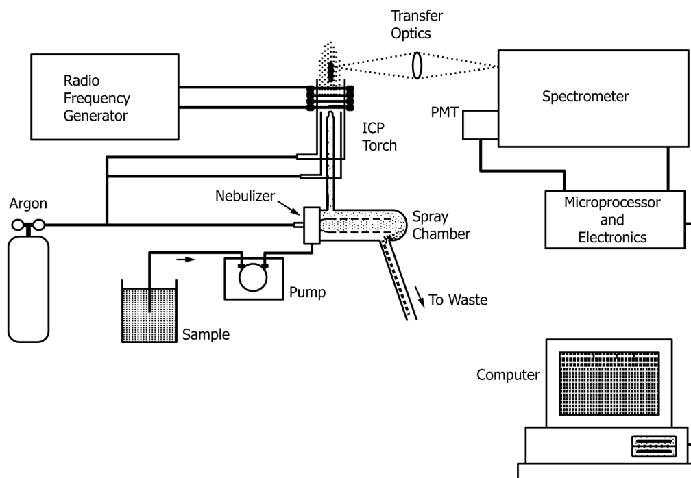
FIG. 1 Components of Inductively Coupled Plasma ICP-AES 4
