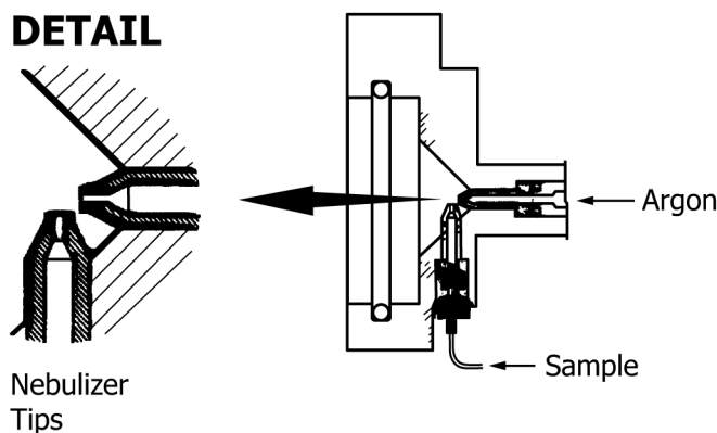
FIG. 4 Cross-Flow Nebulizer 4
