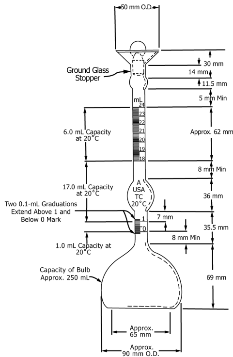
FIG. 1 Le Chatelier Flask for Density Test
