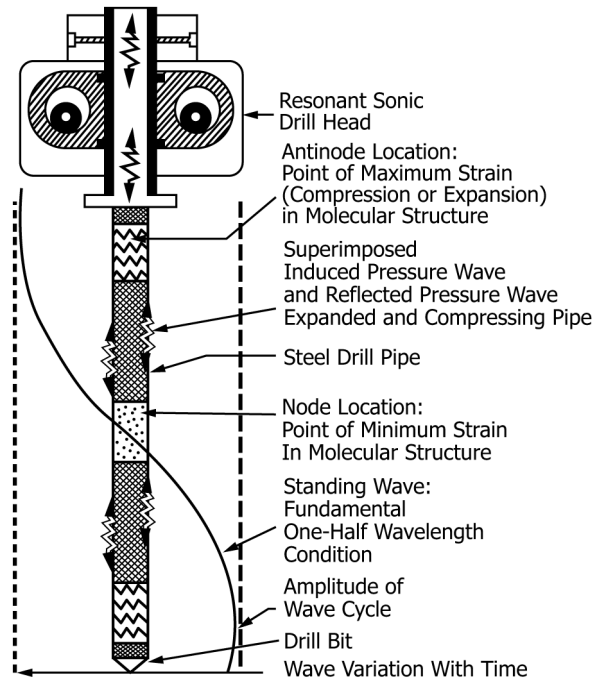
FIG. 1 General Principle of Sonic Drilling
