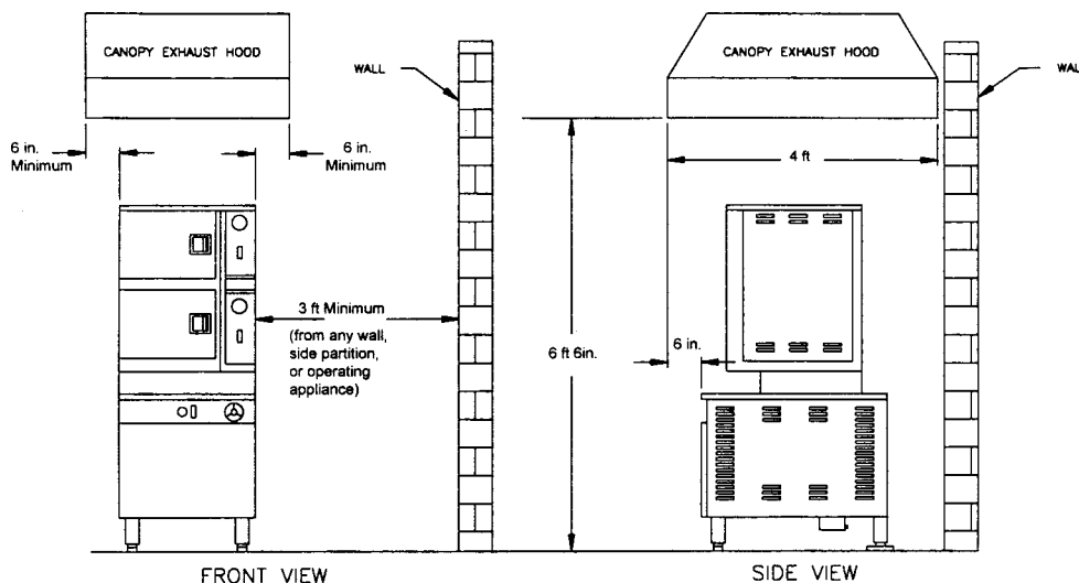
FIG. 2 Equipment Configuration
