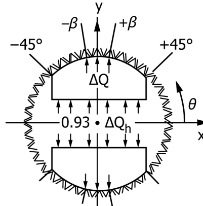
FIG. 2 Schematic of Diametrical Loading of the Borehole JackWall by the Borehole Jack Platens
