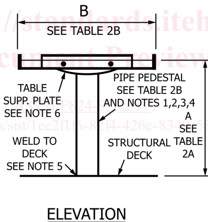
FIG. 2 Square Mess Table (Type II)
