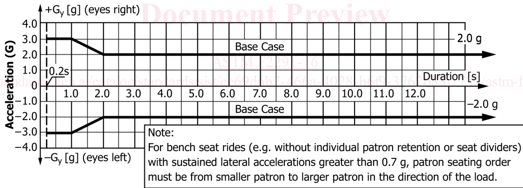
FIG. 7 Acceleration-Duration Limits for -G x (Eyes Front) Gy (Eyes Right and Eyes Left)
