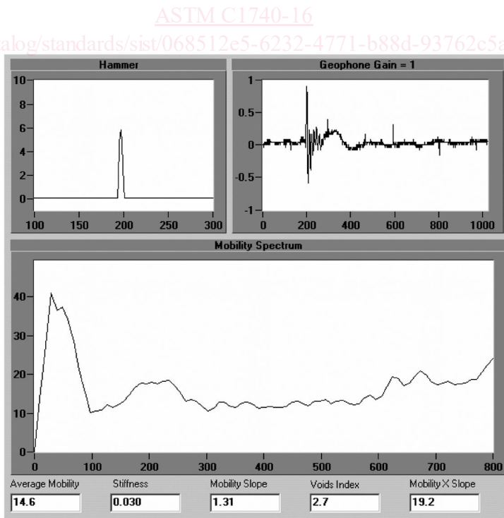
FIG. 5 Invalid Waveform (Upper Right Plot) Caused by Movement of the Velocity Transducer Base
